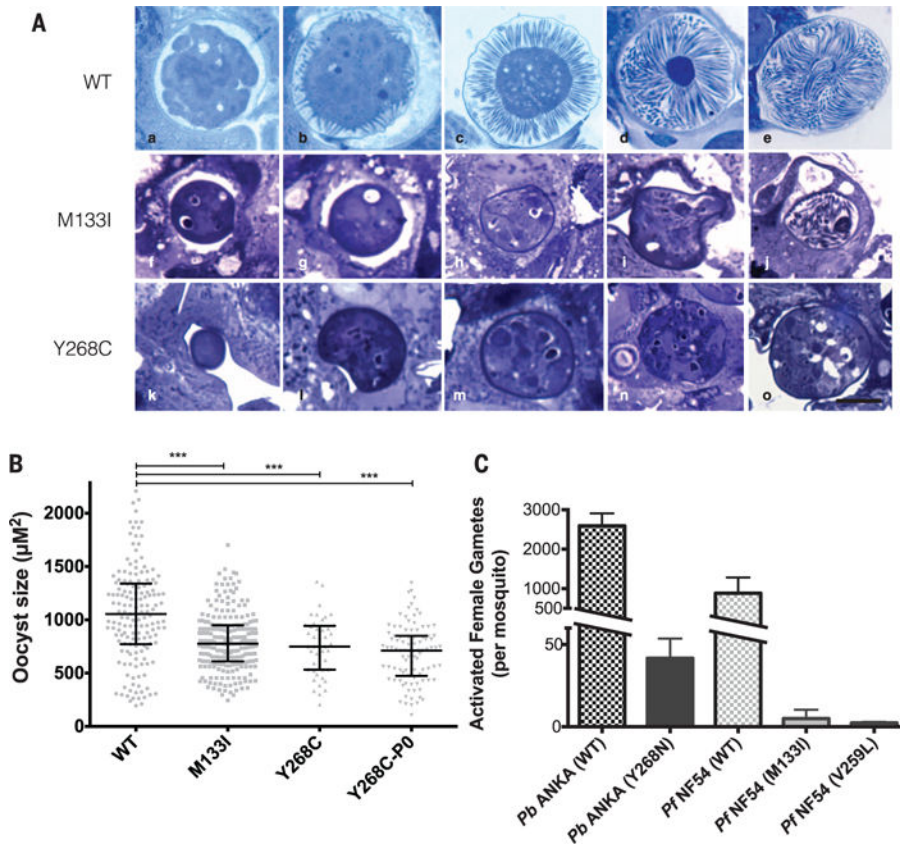
Fig. 1. Atovaquone-resistant parasites generate small, malformed oocysts in the mosquito that fail to form infectious sporozoites
