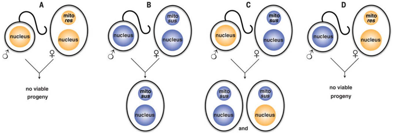
Fig. 2. The genetics of inheritance of mitochondrial DNA–encoded atovaquone resistance mutations in cytB prevent transmission
